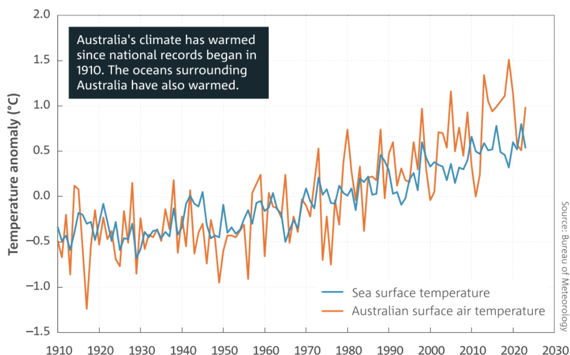
Figure 14: Ocean and surface temperature rises
