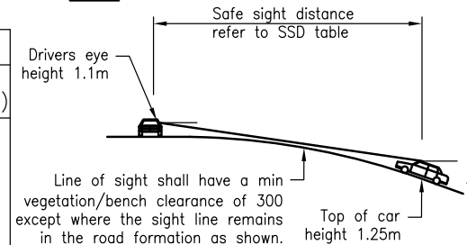
LONGITUDINAL SECTION SSD - EXITING FROM DRIVEWAY
