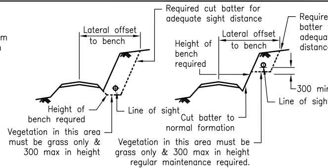
BENCHING DETAIL SECTION B-B
