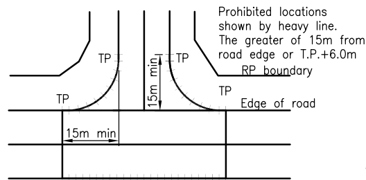
PROHIBITED LOCATIONS AT INTERSECTIONS FOR RURAL DRIVEWAYS
