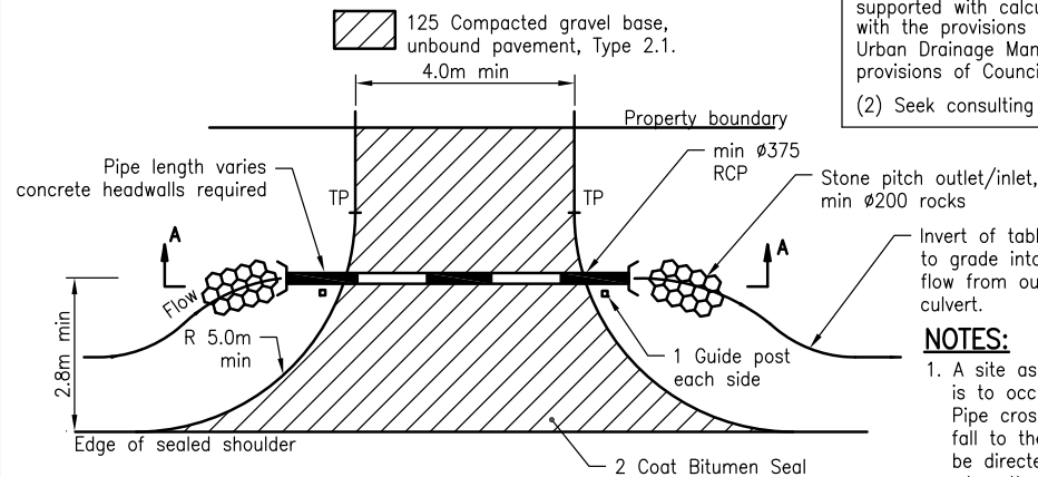
DRIVEWAY PLAN
