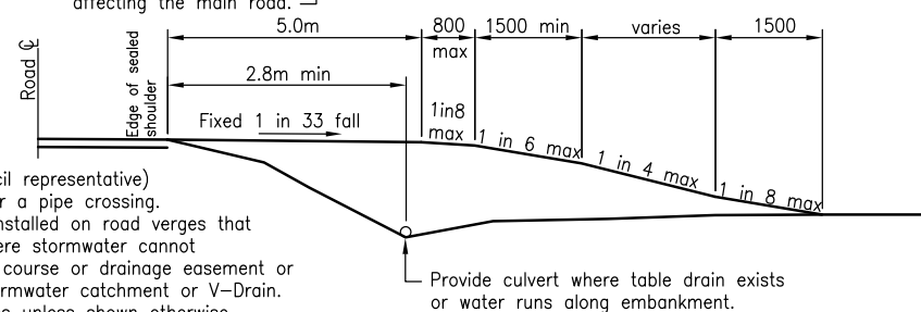
TYPICAL DRIVEWAY SECTION - ROAD IN FILL
