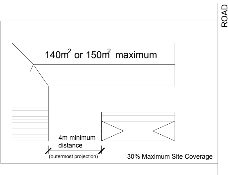
Diagram 4 - Building Setbacks
