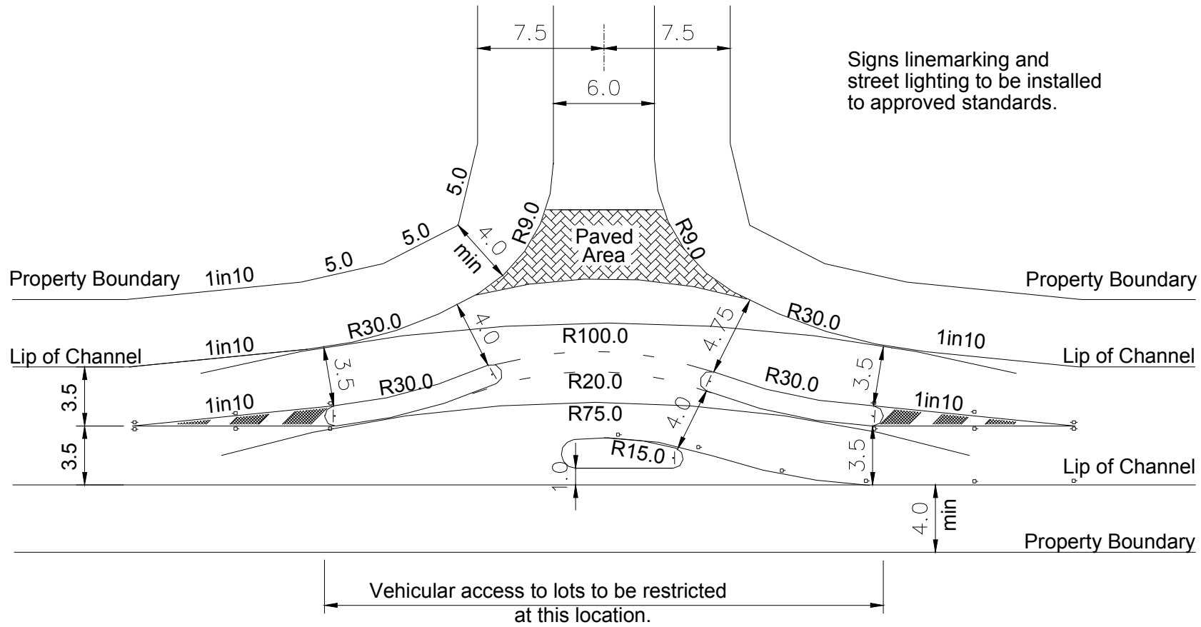
TYPICAL T INTERSECTION SLOW POINT AT JUNCTION OF TYPE A TO B STREETS GUIDE ONLY
